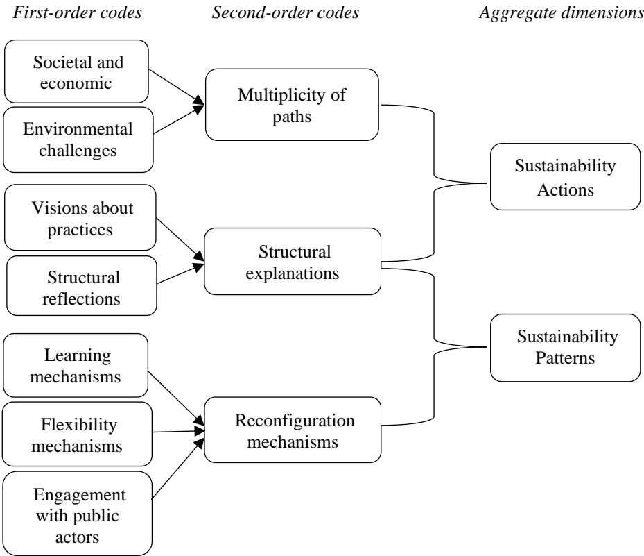
Figure 1 : Data structure
